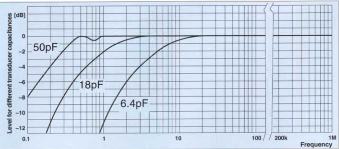
Fig. 1: Frequency response of preamplifier type 1201 for different source impedances.
