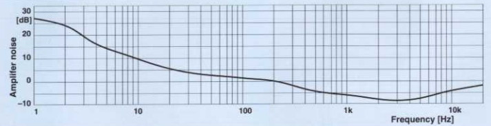
Fig. 2: Amplifier noise for 18pF source impedance in 1/3 octave bands.
